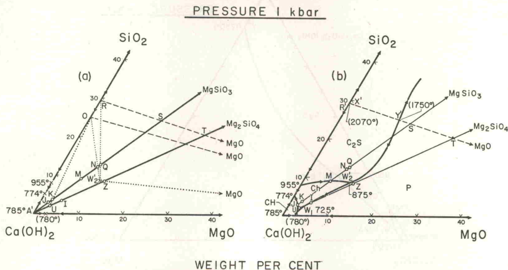
Fig. 5. Phase relationships on the vapor-saturated liquidus surface when projected onto the triangle Ca(OH) 2 -MgO-SiO 2 , as constructed from the experimental results in Fig. 4. Note the line RST MgO in Figs. 1 and 3.
